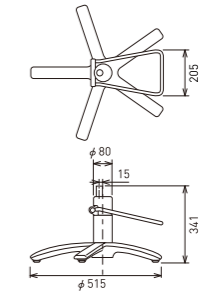
SP-YA Chrome Initial height:341mm Stroke:142mm
