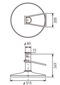
SP-YE Hairline Initial height:349mm Stroke:142mm
